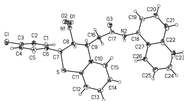
Figure 1. X-ray crystal structure of 6 .
